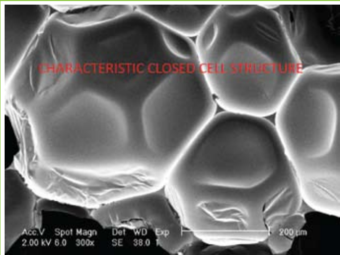
Scanning Electron Microscope picture c/o Sophie Reynolds, Birmingham University
